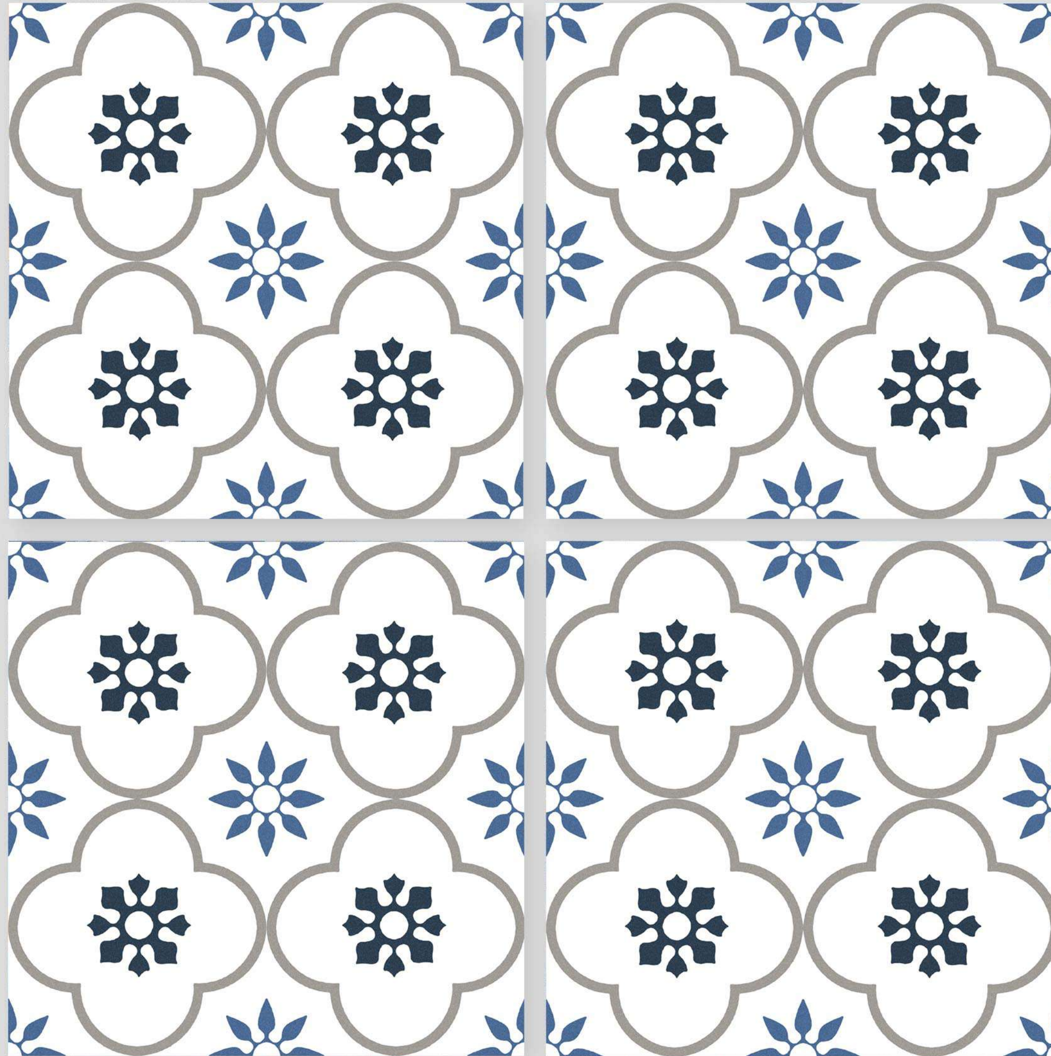
Random
